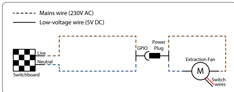
Image 2: Functional wiring diagram showing fan (no switch) connection for a bathroom
