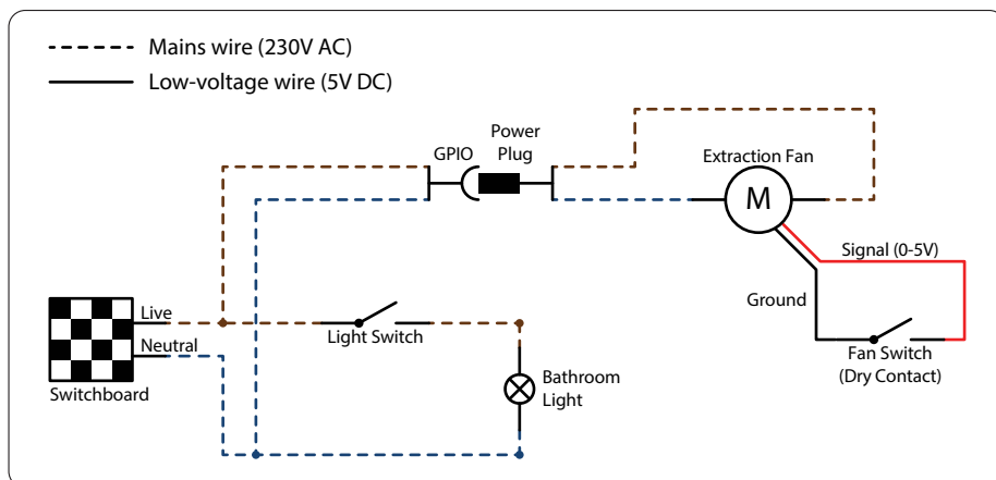
Image 1: Functional wiring diagram showing fan and switch connection for a bathroom
